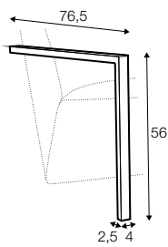
wood frame
